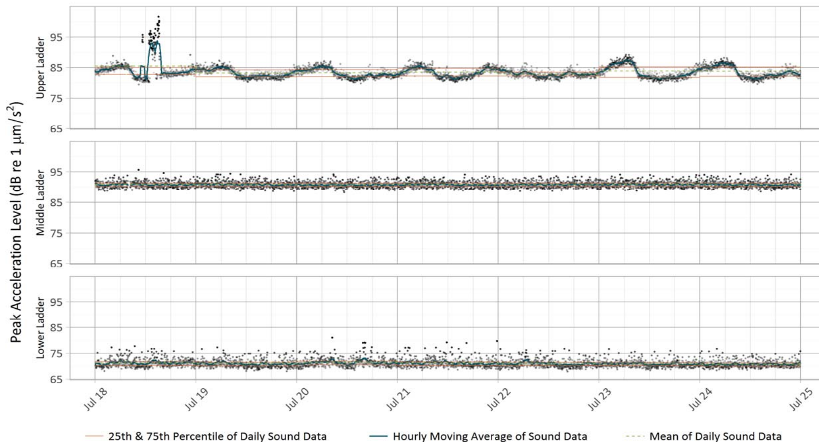
Figure 1 Peak Acceleration Levels Measured by Triaxial Accelerometers for Week 29
